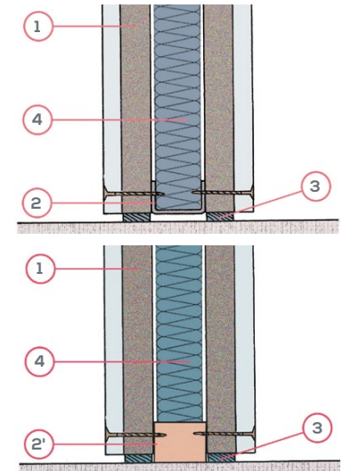
Extension essai CEDIA 2011/5862
